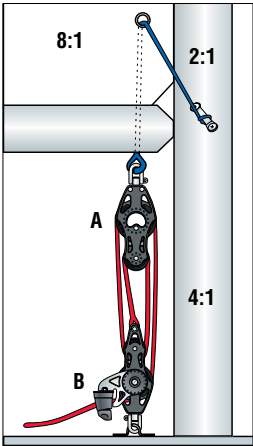
8:1 Cascaded: The most basic cunningham is a self-cleating 8:1 tackle positioned at the mastbase.
