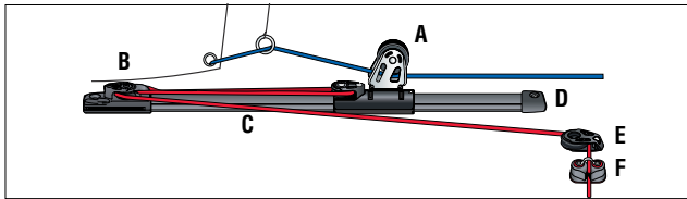
Barbarhailer: Use this low-profile system on racing boats with nonoverlapping jibs like the Farr® 40 and One Design 35. An inhaul is used to control slot size.
