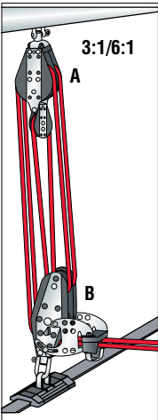
3:1/6:1: This 3:1/6:1 two-speed system is used on end-boom sheeting and mainsails up to 22.3 m 2 (240 ft 2 ).
