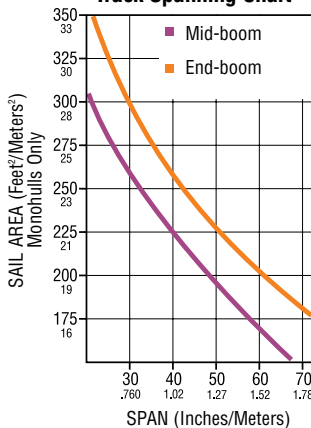
27 mm High-Beam Track Spanning Chart
