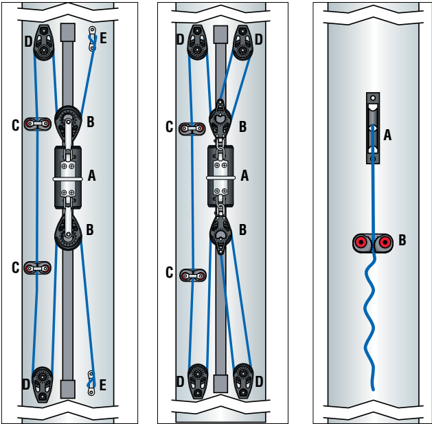
2:1 Spinnaker Pole: This system allows the inboard end of the pole to be moved under load. It features a continuous adjuster line and 2:1 controls.
